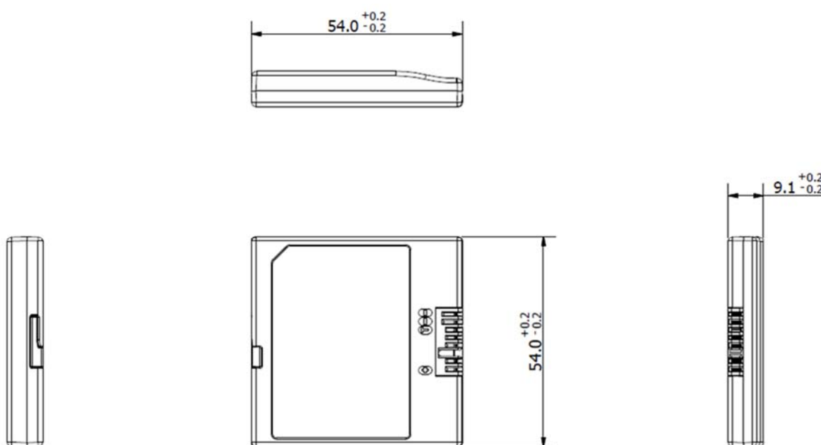
Figure 6 - Battery Dimensions
