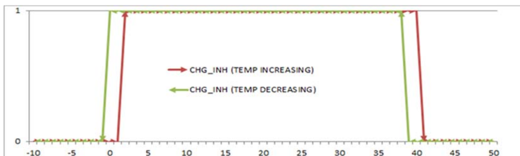
Figure 4 - CHG_INH Operation
